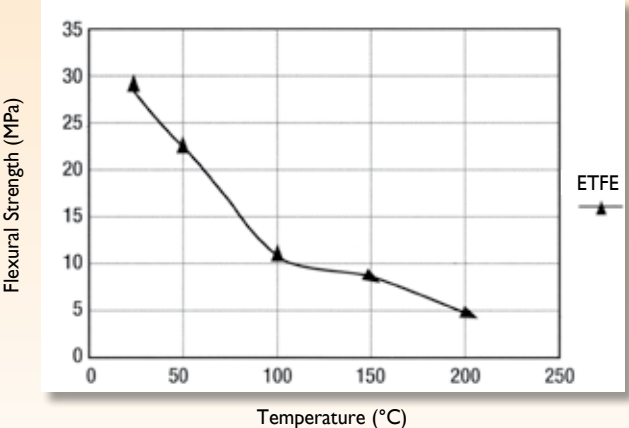
Effect of Temperature on Flexural Strength
